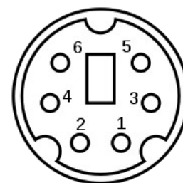
Front view of miniDIN6 male connector
