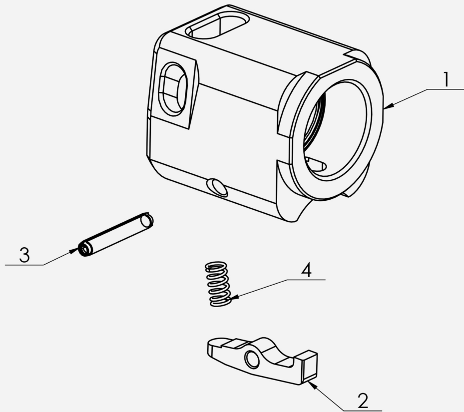
Self Indexing Compensator Parts List
