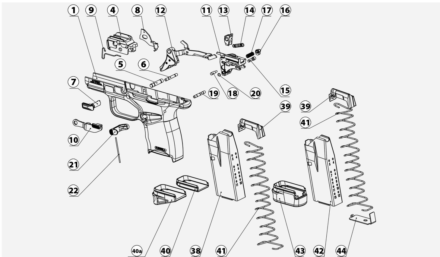
Hellcat Frame Parts List
