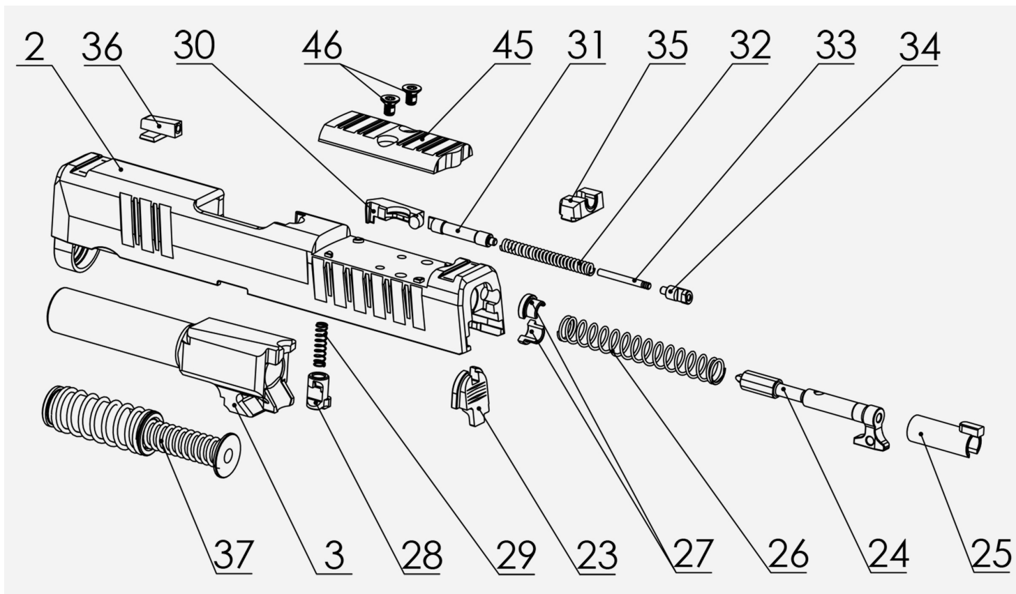
Hellcat OSP Slide Parts List
