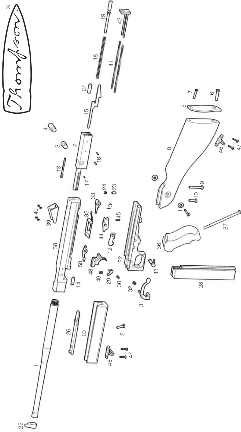
EXPLODED VIEW, MODELS: TM1, TM1C and M1SB
